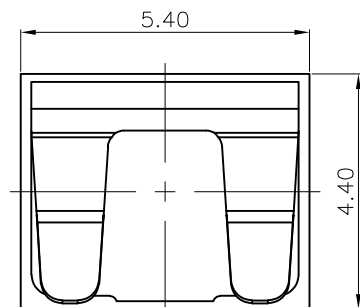
RECOMMENDED PCB LAYOUT S=10:1
